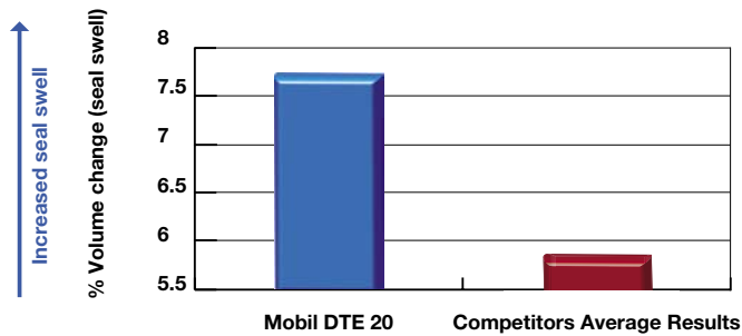
ISO VG 46 Hydraulic Oil in seal swell test NBR-1, 100°C, 168 hrs (run under DIN conditions)
