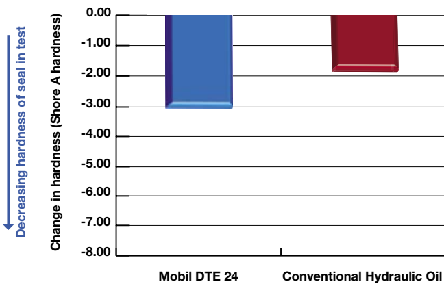
Seal Compatibility 168 hrs, 100°C, NBR -1, Shore A Hardness Run under DIN conditions
